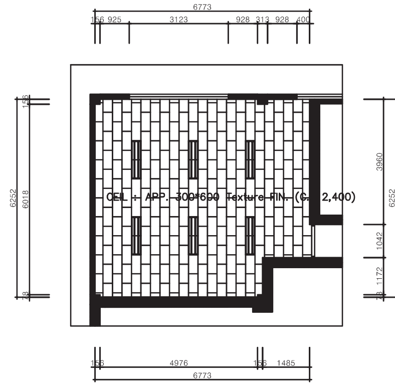
CEILING PLAN
