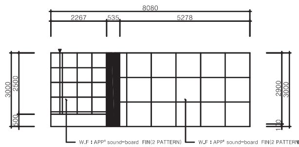
ELEVATION_B-B'
