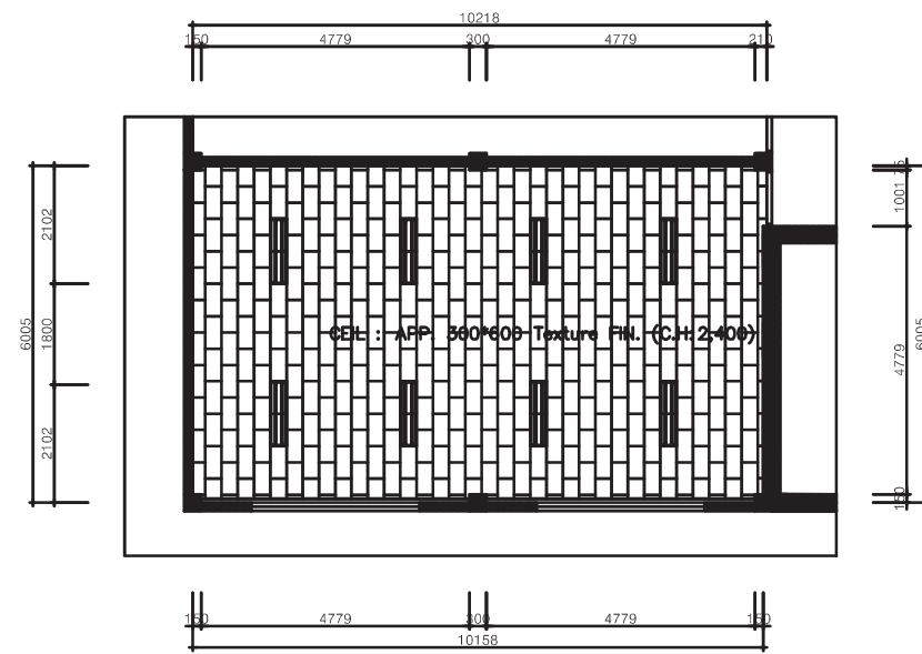
CEILING PLAN
