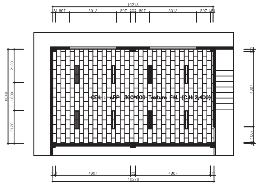
CEILING PLAN
