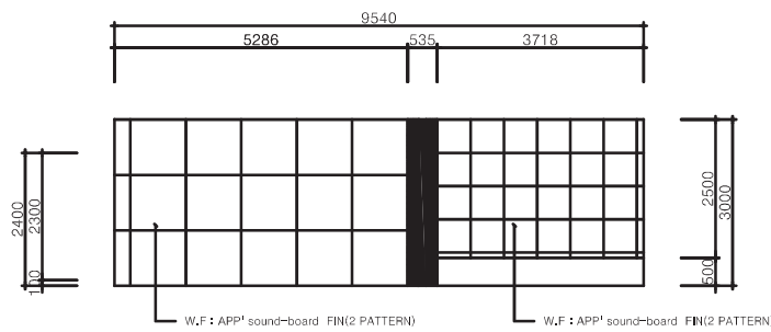
ELEVATION_A-A'
