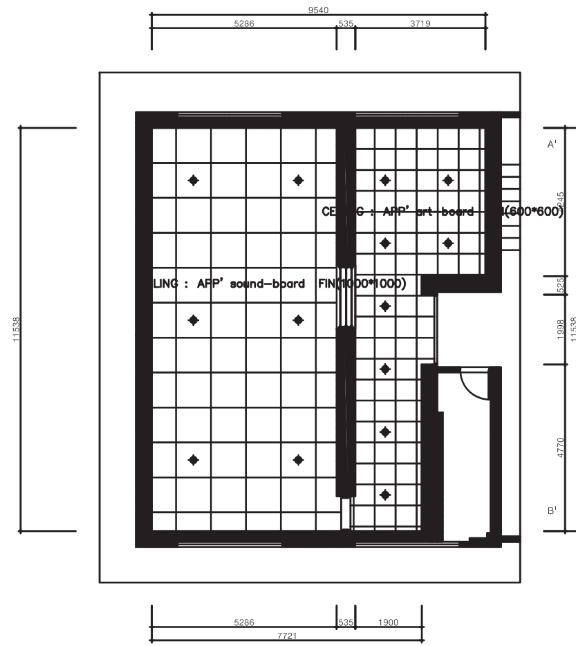
CEILING PLAN
