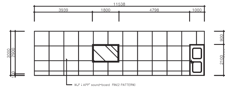
ELEVATION_E
