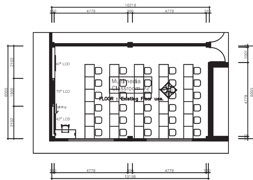
FLOOR PLAN
