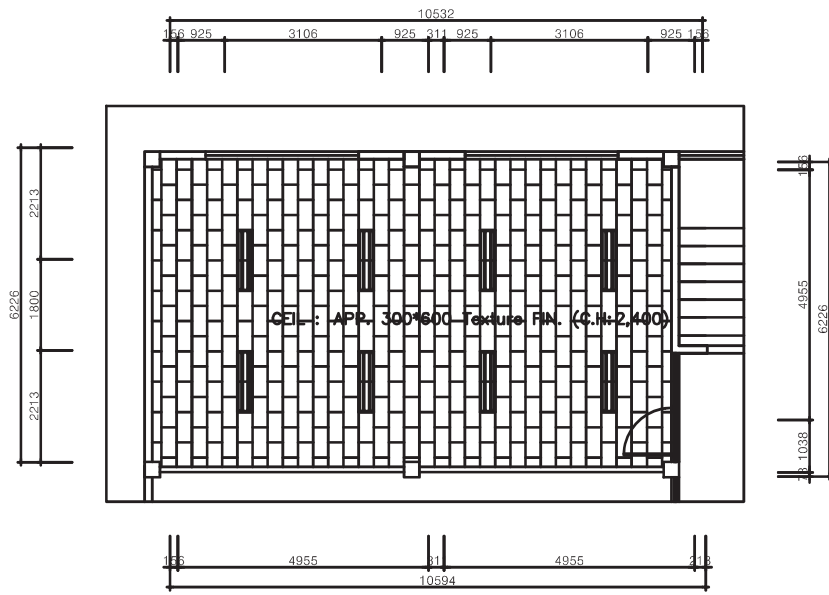
CEILING PLAN
