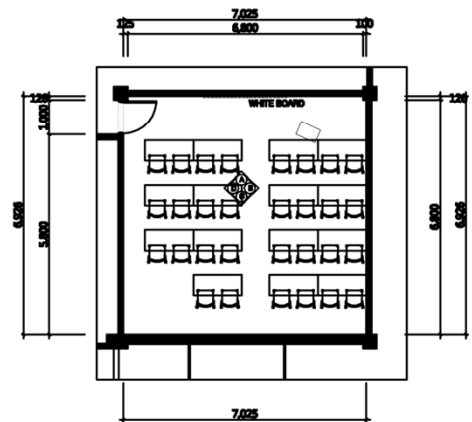
FLOOR PLAN
