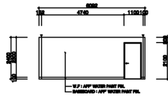
ELEVATION_A/B
