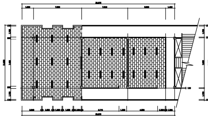
CEILING PLAN
