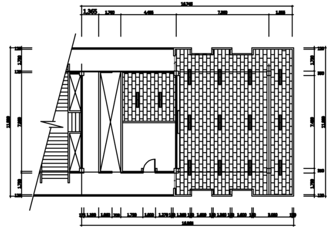
CEILING PLAN
