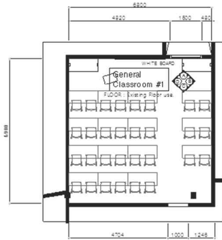
FLOOR PLAN
