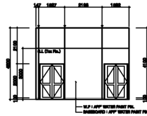
ELEVATION_A/B
