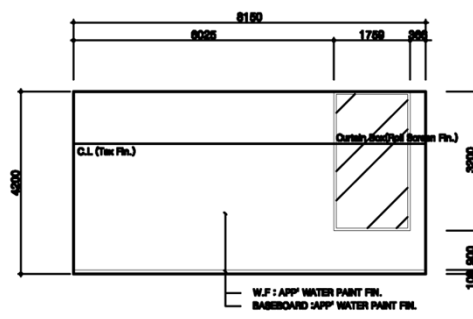
ELEVATION_C/D
