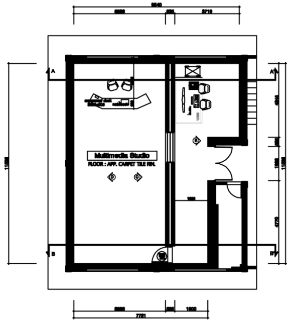
FLOOR PLAN
