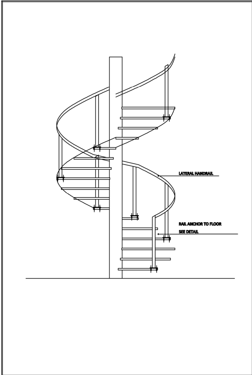
SPIRAL STAIRCASE DETAILS
