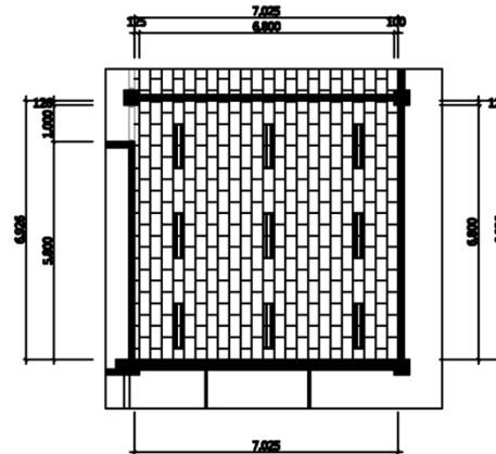
CEILING PLAN
