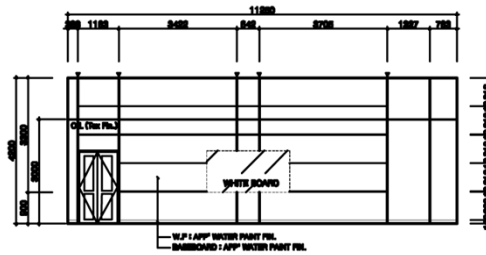
ELEVATION_C/D
