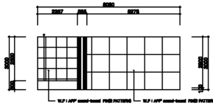
ELEVATION_B-B'
