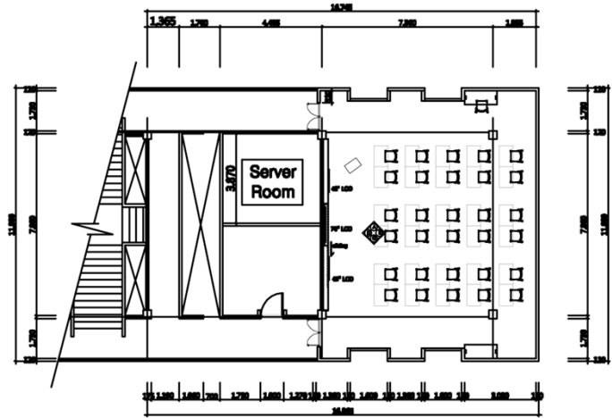
FLOOR PLAN
