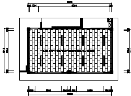
CEILING PLAN
