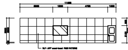
ELEVATION_E
