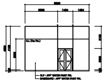
ELEVATION_A/B
