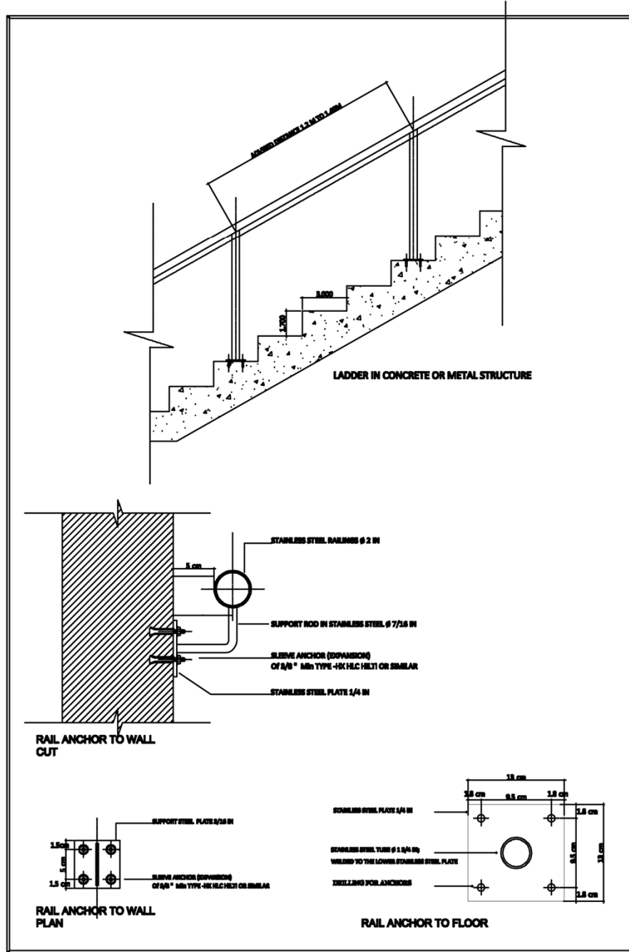
STAIR DETAILS
