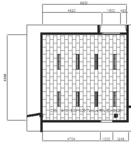
CEILING PLAN
