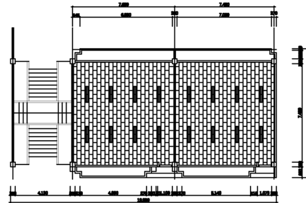
CEILING PLAN
