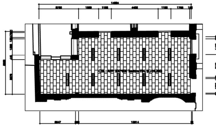
CEILING PLAN
