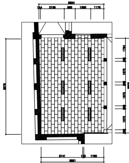
CEILING PLAN
