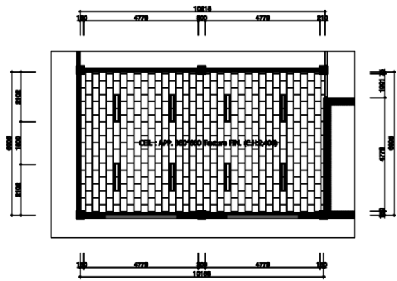
CEILING PLAN
