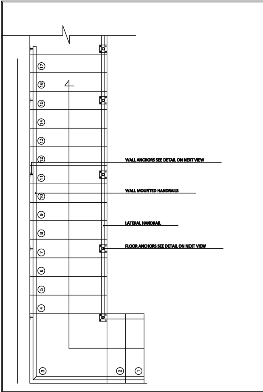
STAIR DETAILS
