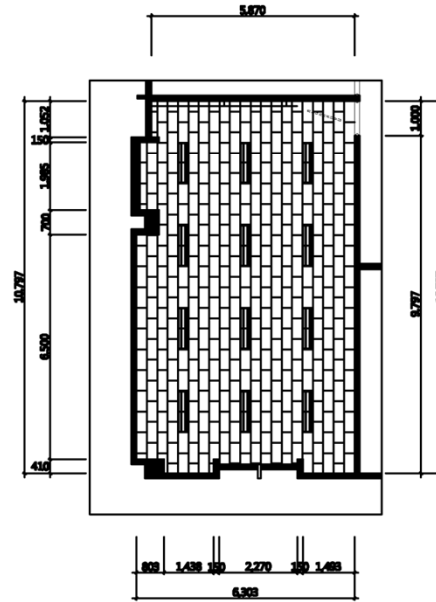
CEILING PLAN
