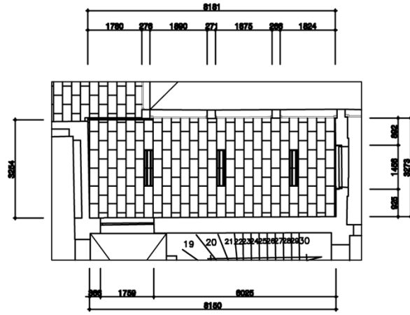
CEILING PLAN
