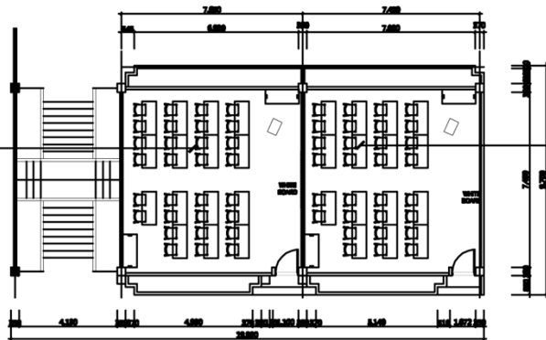
FLOOR PLAN
