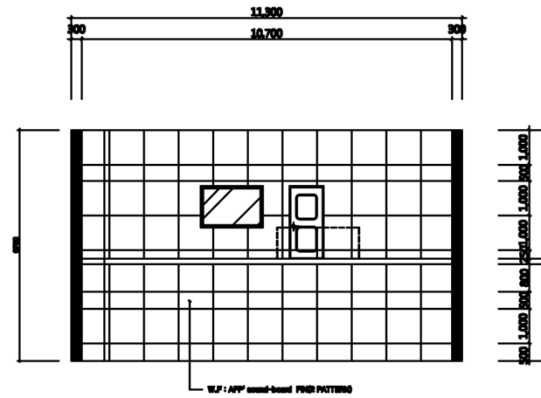
ELEVATION_A/B
