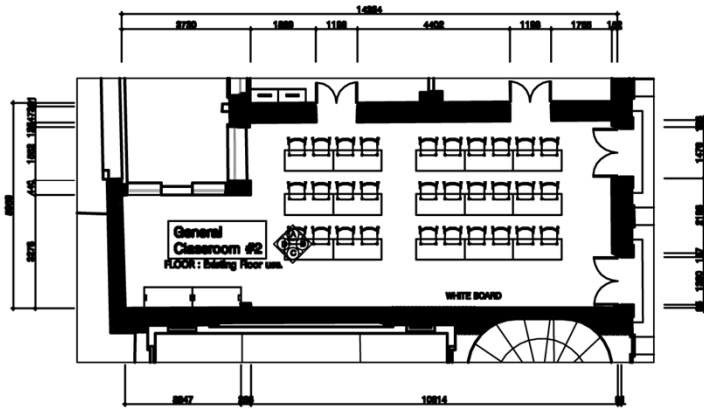
FLOOR PLAN
