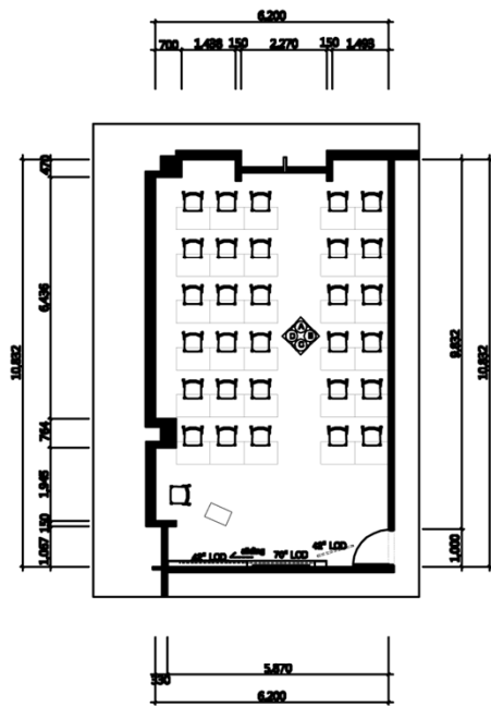
FLOOR PLAN
