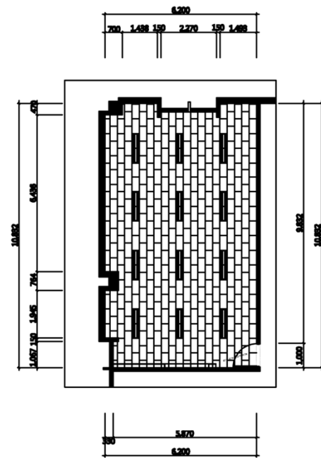
CEILING PLAN
