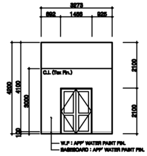
ELEVATION_A/B
