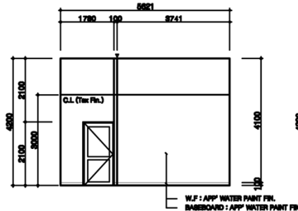
ELEVATION_C/D
