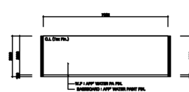
ELEVATION_C/D
