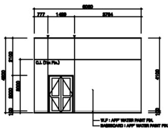
ELEVATION_A/B
