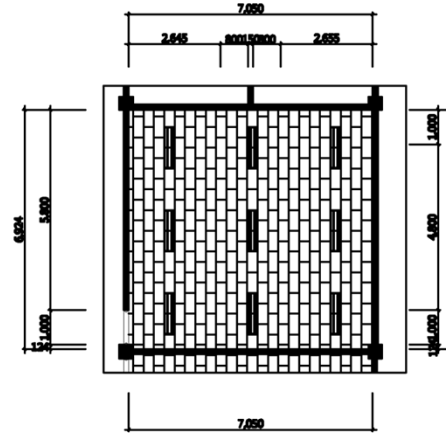
CEILING PLAN
