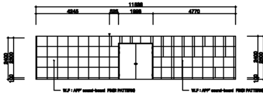
ELEVATION_C
