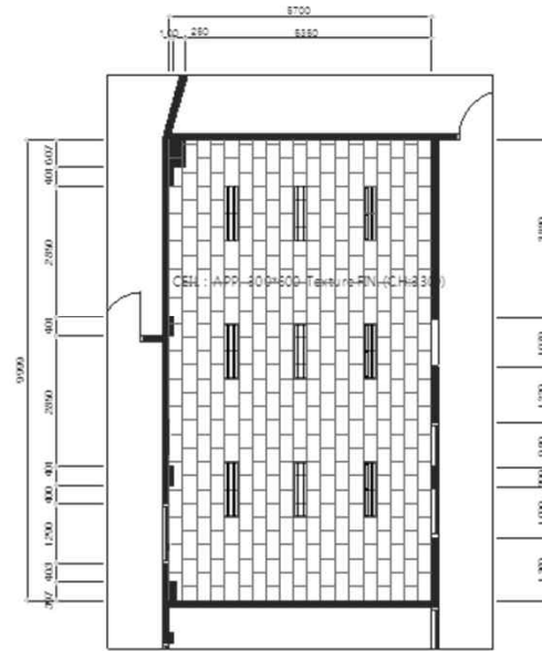
CEILING PLAN
