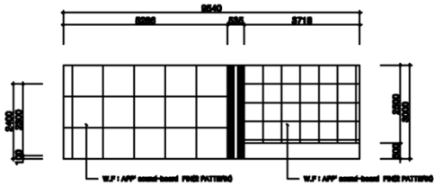
ELEVATION_A-A'
