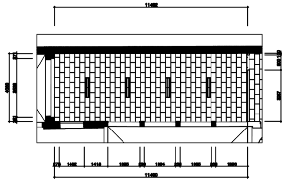
CEILING PLAN
